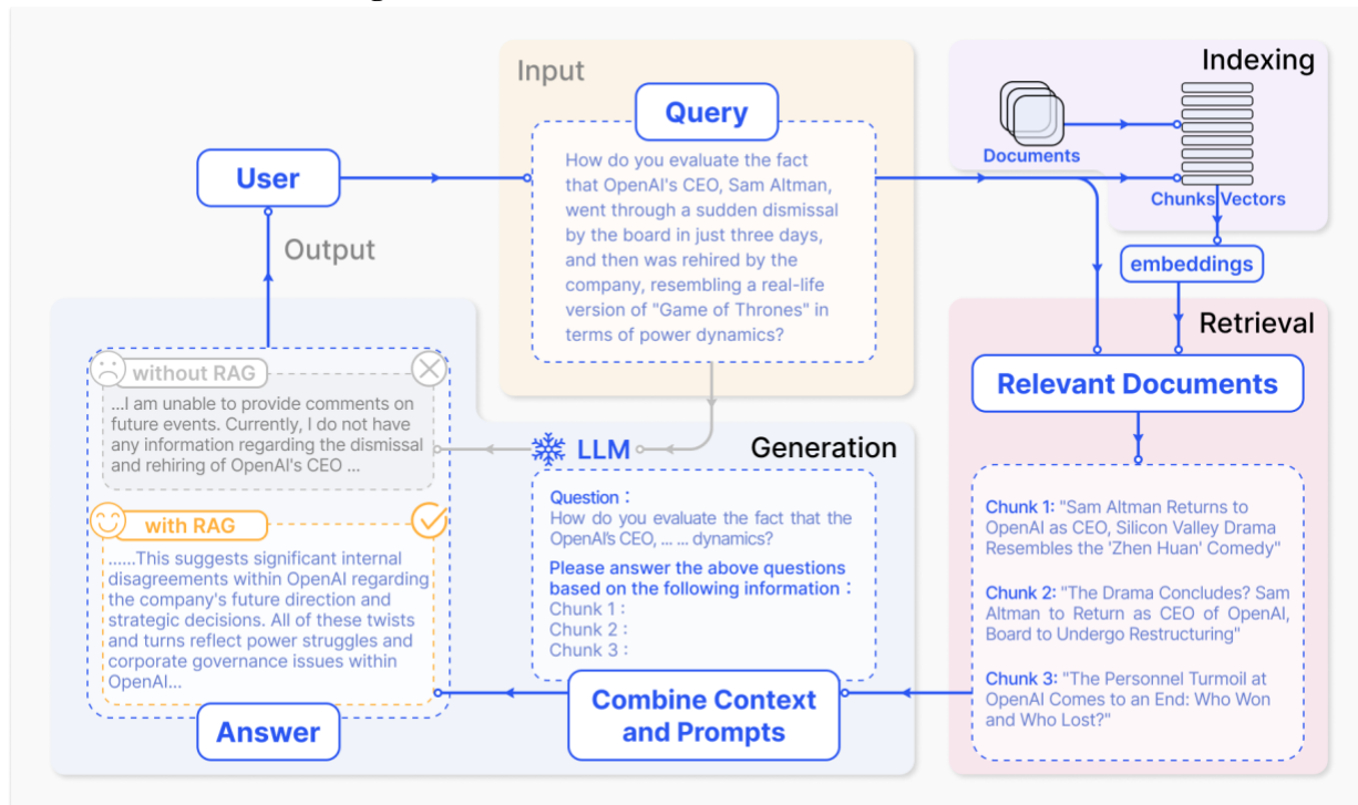
FIGURE 13. Retrieval Augmented Generation (RAG) workflow
