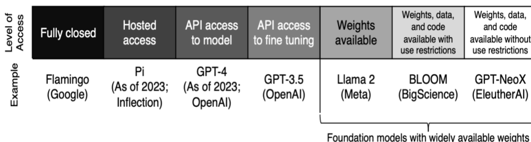
FIGURE 5. A revised spectrum of closed- to open-source models
